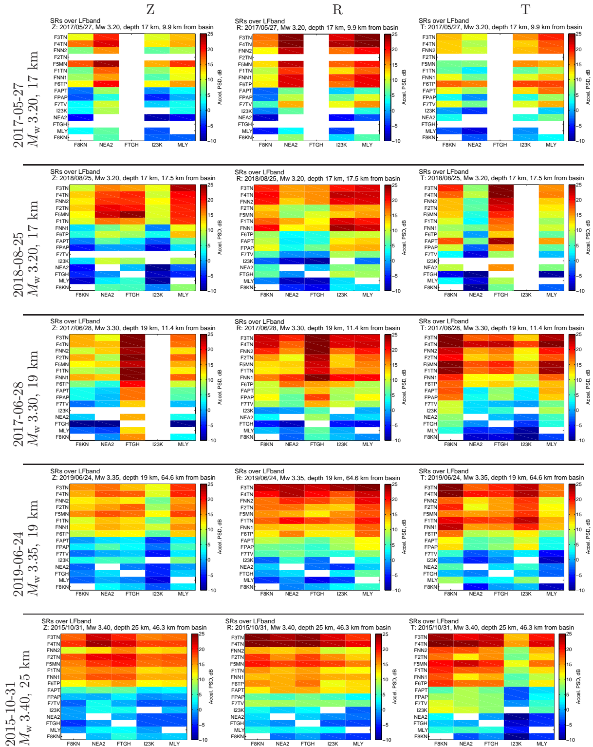
Figure SR1: LFband : Local and regional spectral ratios sorted by increasing magnitude . The vertical axis is sorted by descending SR's reference station F8KN in the transverse component from Figure 5 of Smith and Tape (2020). The horizontal axis is sorted by median distance to all local events.
