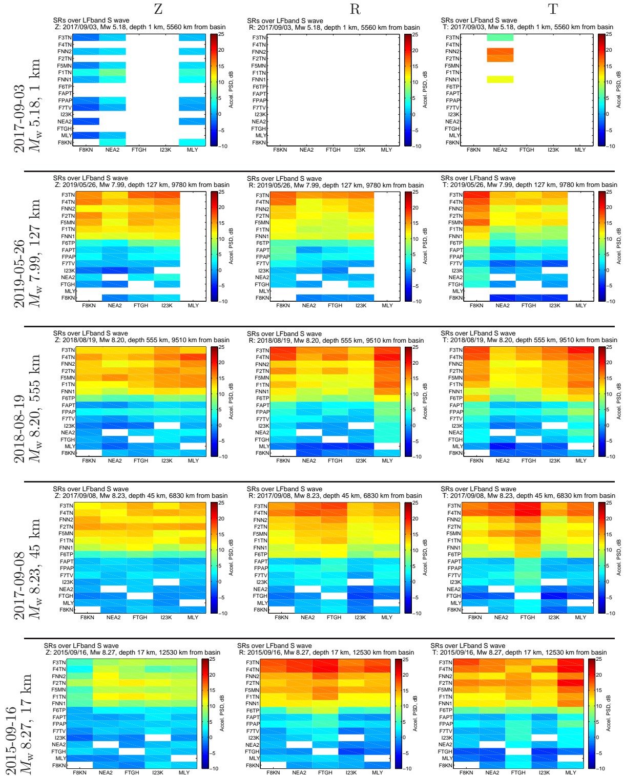
Figure SR11: LFband: Teleseismic S wave spectral ratios sorted by increasing magnitude . The vertical axis is sorted by descending SR's reference station F8KN in the transverse component in Figure 5. The horizontal axis is sorted by median distance to all local events.
