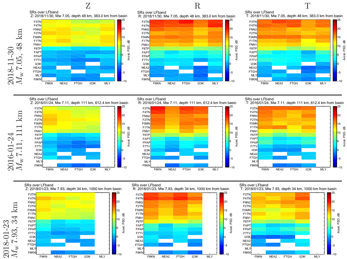
Figure SR9: LFband : Local and regional spectral ratios sorted by increasing magnitude . The vertical axis is sorted by descending SR's reference station F8KN in the transverse component from Figure 5 of Smith and Tape (2020). The horizontal axis is sorted by median distance to all local events.
