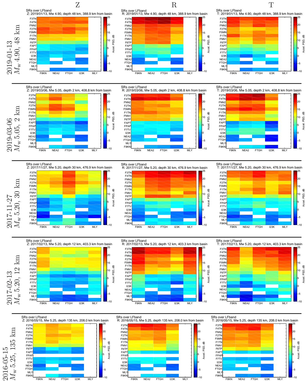
Figure SR7: LFband : Local and regional spectral ratios sorted by increasing magnitude . The vertical axis is sorted by descending SR's reference station F8KN in the transverse component from Figure 5 of Smith and Tape (2020). The horizontal axis is sorted by median distance to all local events.
