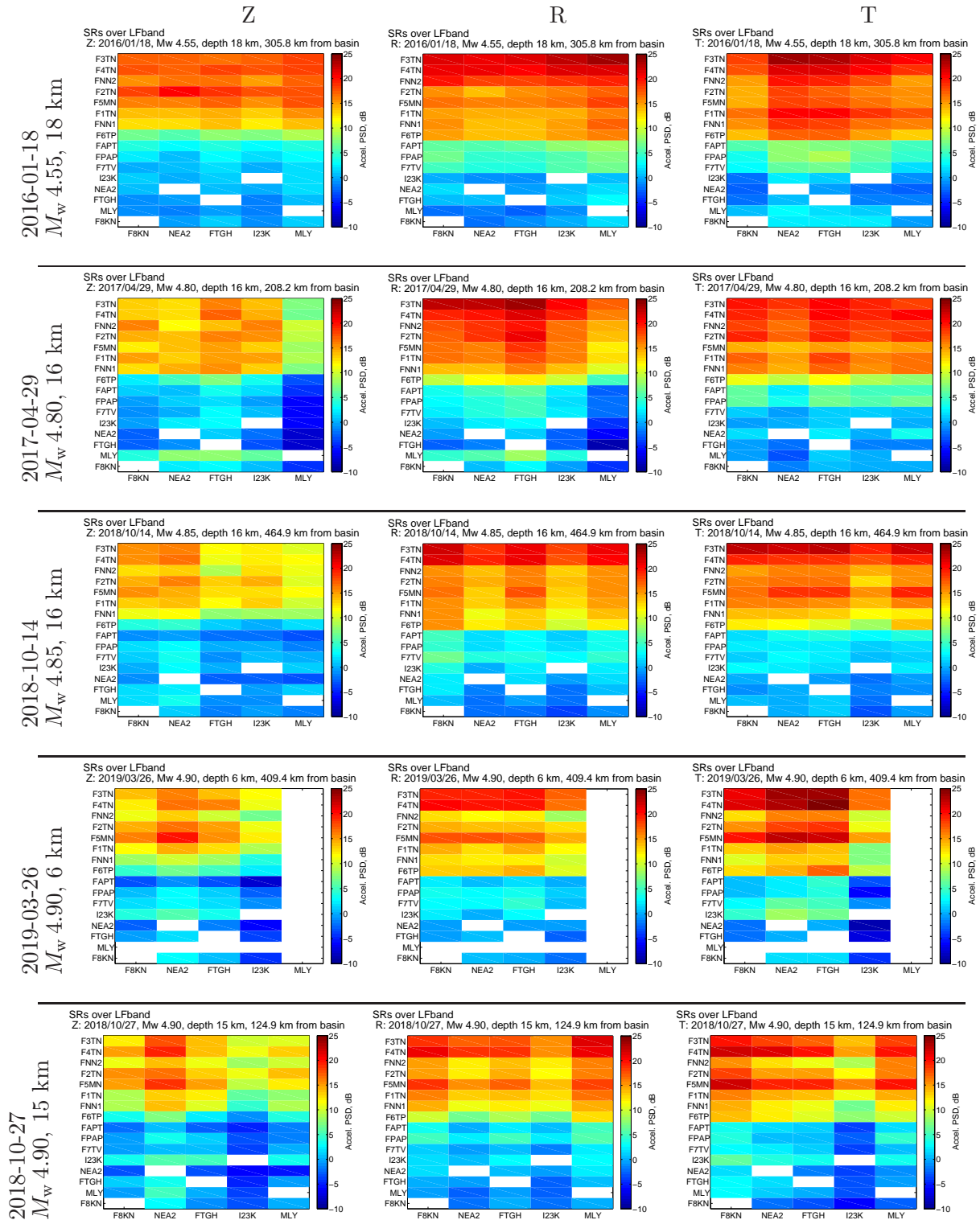
Figure SR6: LFband : Local and regional spectral ratios sorted by increasing magnitude . The vertical axis is sorted by descending SR's reference station F8KN in the transverse component from Figure 5 of Smith and Tape (2020). The horizontal axis is sorted by median distance to all local events.
