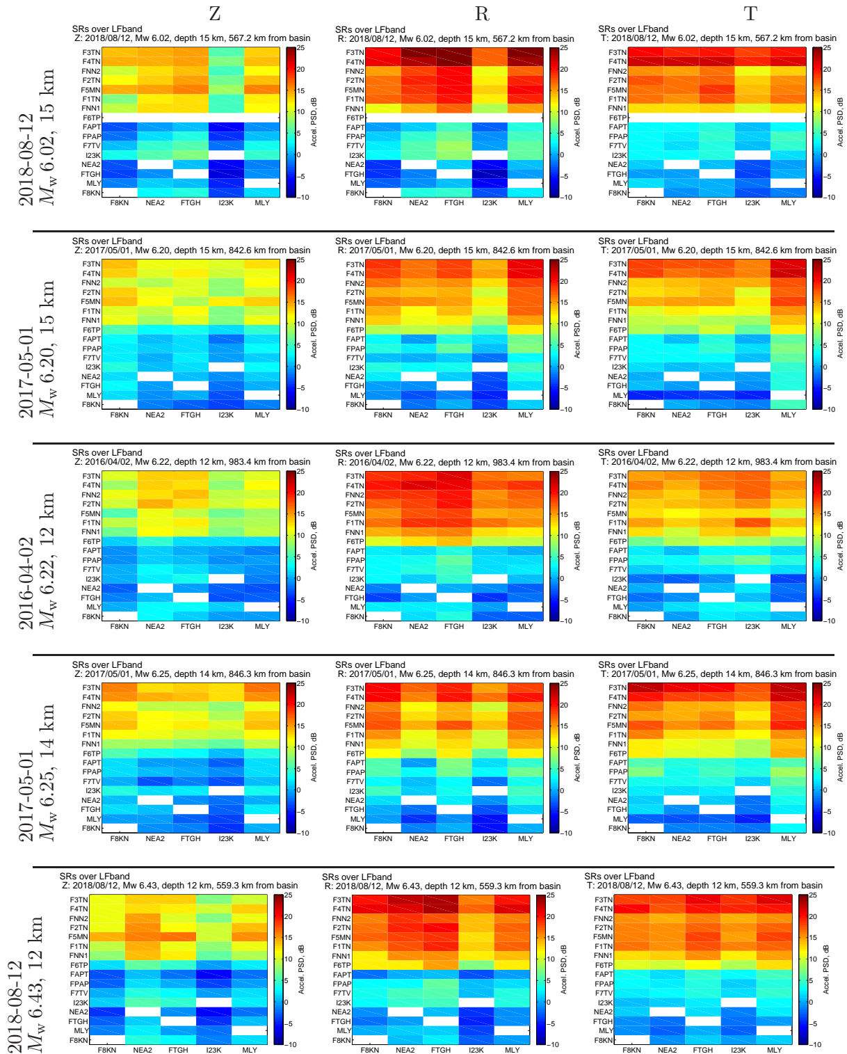
Figure SR8: LFband : Local and regional spectral ratios sorted by increasing magnitude . The vertical axis is sorted by descending SR's reference station F8KN in the transverse component from Figure 5 of Smith and Tape (2020). The horizontal axis is sorted by median distance to all local events.
