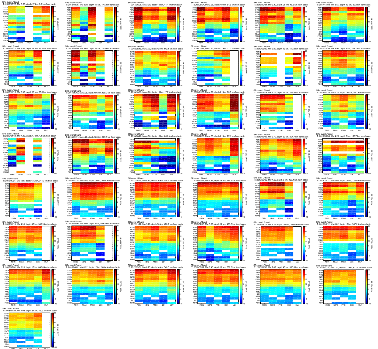
Figure SR14: T: LFband. Events sorted by Table 1 of Smith and Tape (2020).
