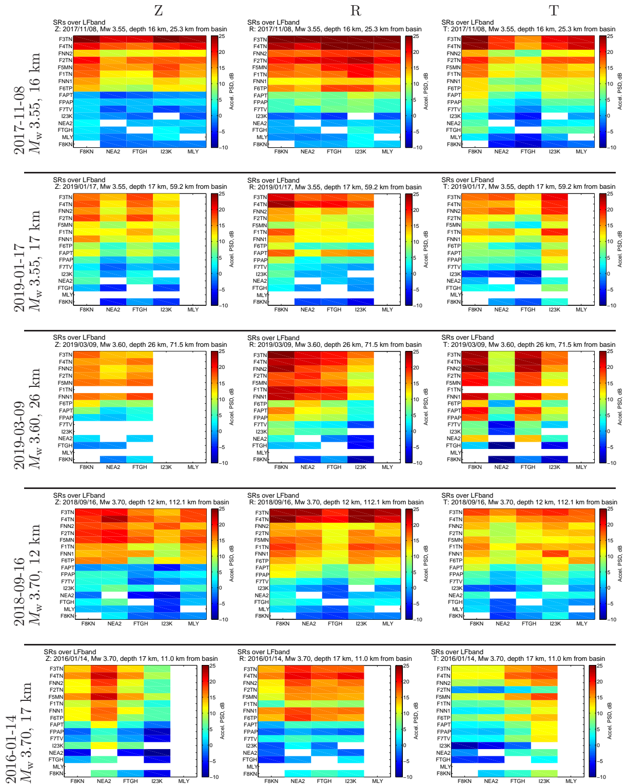
Figure SR2: LFband : Local and regional spectral ratios sorted by increasing magnitude . The vertical axis is sorted by descending SR's reference station F8KN in the transverse component from Figure 5 of Smith and Tape (2020). The horizontal axis is sorted by median distance to all local events.
