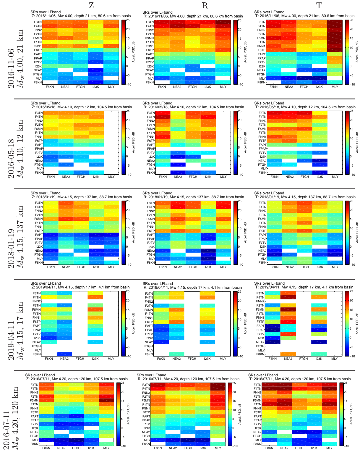
Figure SR4: LFband : Local and regional spectral ratios sorted by increasing magnitude . The vertical axis is sorted by descending SR's reference station F8KN in the transverse component from Figure 5 of Smith and Tape (2020). The horizontal axis is sorted by median distance to all local events.
