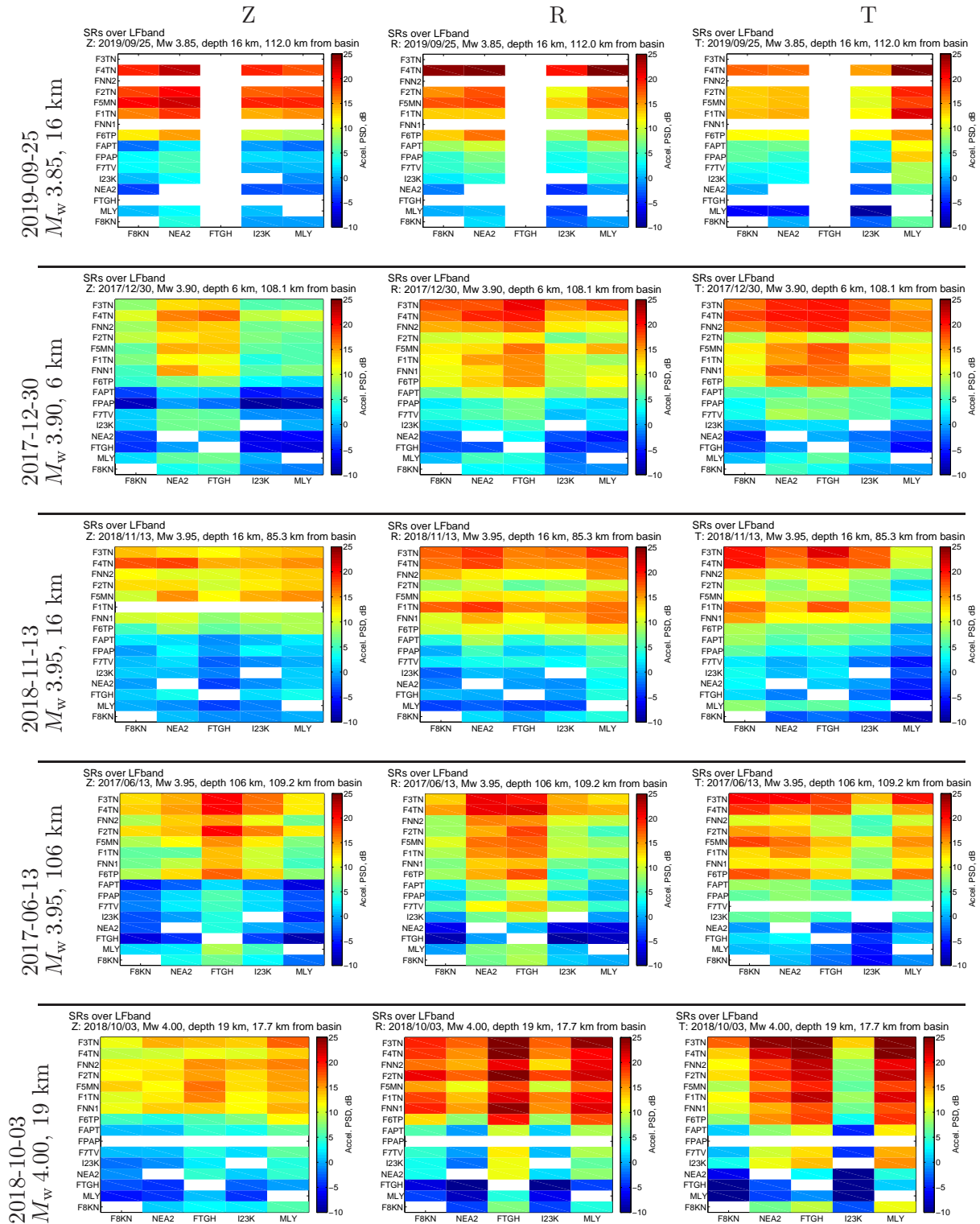
Figure SR3: LFband : Local and regional spectral ratios sorted by increasing magnitude . The vertical axis is sorted by descending SR's reference station F8KN in the transverse component from Figure 5 of Smith and Tape (2020). The horizontal axis is sorted by median distance to all local events.
