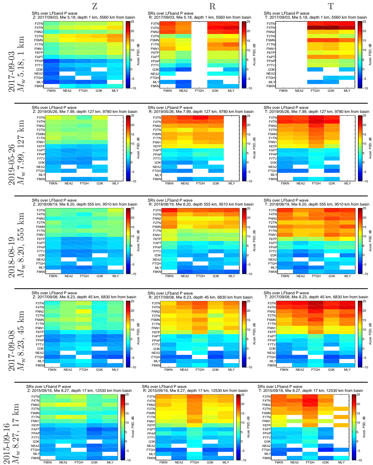
Figure SR10: LFband: Teleseismic P wave spectral ratios sorted by increasing magnitude . The vertical axis is sorted by descending SR's reference station F8KN in the transverse component in Figure 5. The horizontal axis is sorted by median distance to all local events.
