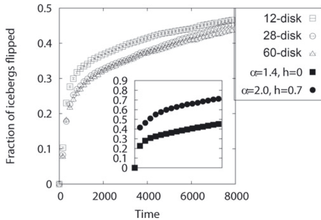
Fig. 2. The fraction of icebergs capsized by at least 45^\circ as a function of time for a 12-, 28- and 60-disk representation for the \alpha_o = 1.4 , h = 0 ice shelf. Each curve is averaged over eight simulation runs with different initial conditions. The error bars are determined from the standard deviation of the simulation results at each time. The inset shows a comparison between the \alpha_o = 1.4 , h = 0 and the \alpha_o = 2.0 , h = 0.7 iceberg assemblages, using the same scale on the x-axis.
