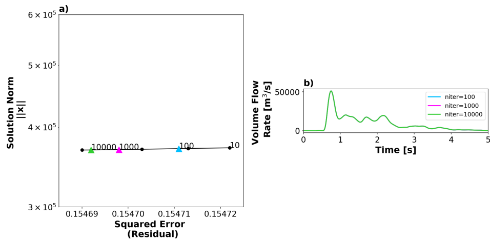
Figure 1. Monopole inversion stability test. (a) Convergence curve of the norm of the solution ( \|x\| ) and squared error (residual) with respect to number of iterations for example event YBAL.3A8. (b) Volume flow rate solution as a function of time for 100 (blue), 1000 (pink), and 10000 (green) iterations. Blue, pink and green triangles in (a) correspond to volume flow rate vectors plotted in (b).
