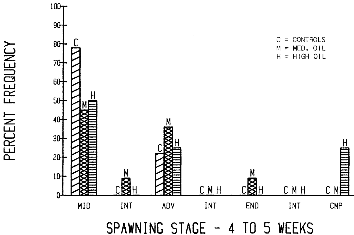
Fig. 9. Comparison of study populations to show frequency of animals in each spawning stage. MID = Mid Spawning; INT. = Inter-stage; ADV. = Advance Spawning; END = End Spawning; CMP = Completed Spawning.
