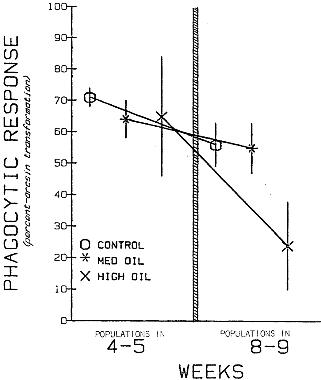
Fig.7. Phagocytic response to yeast. Population means and 95% confidence of percentage changes as a result of time and exposure to 500 and 1000 nL/L of oil. Number of animals sampled: Controls = 9,11; Med. oil = 11,12; High oil = 4,5.
