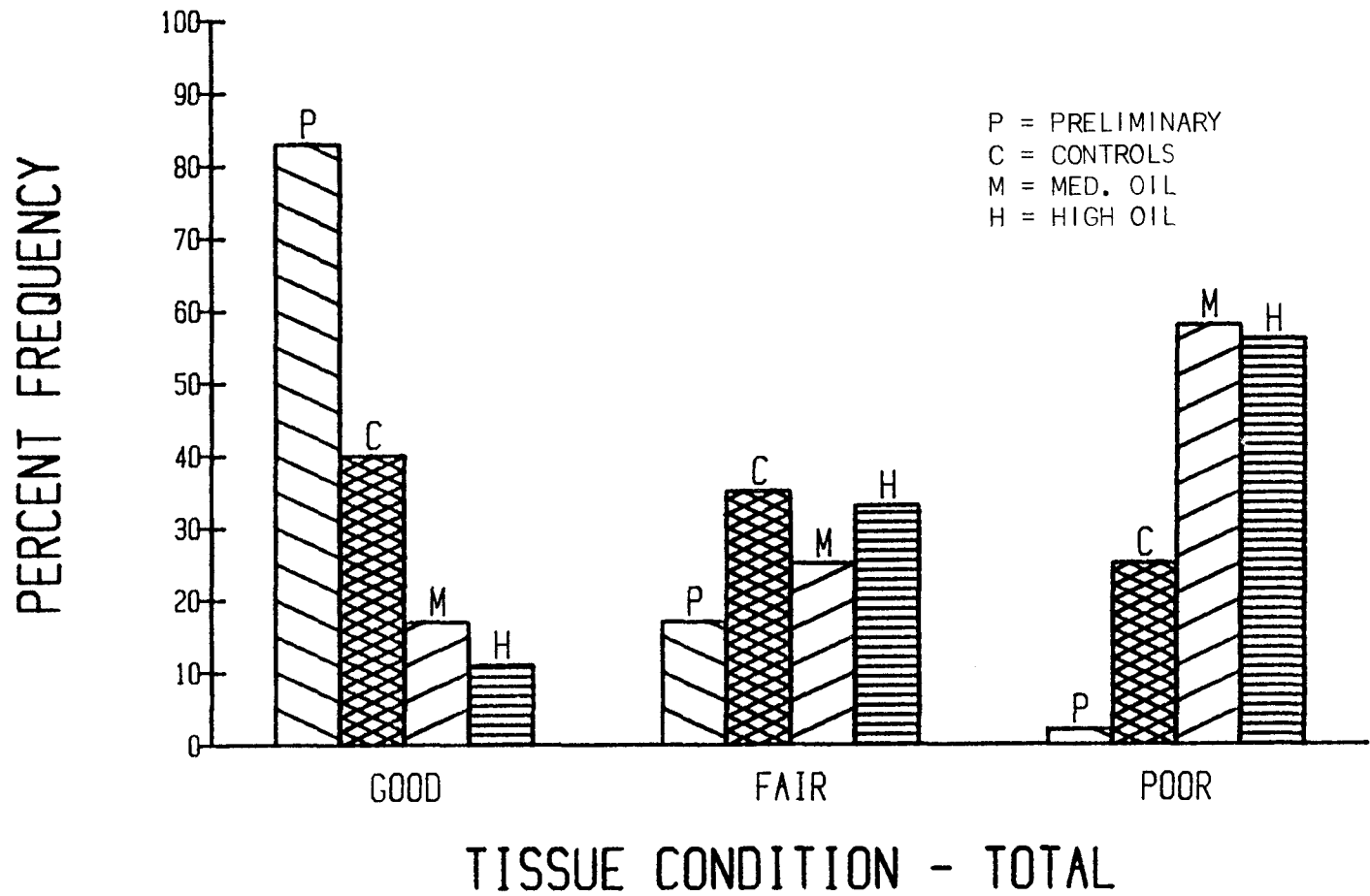
Fig. 11. Comparison of all study populations and the percent frequency of all animals classed as Good, Fair, or Poor condition.
