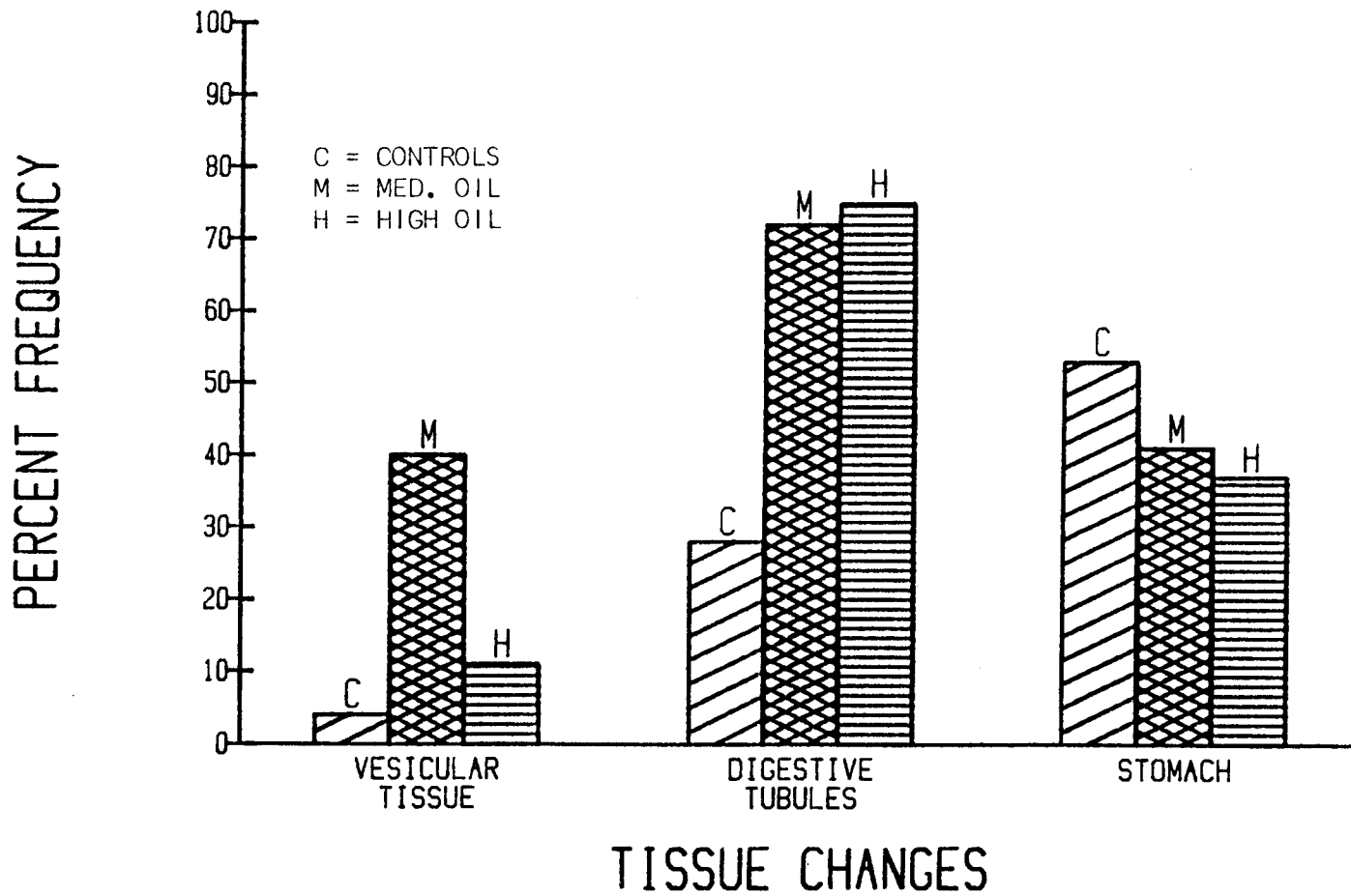
Fig. 13. Comparison of study populations and percent frequency of animals with structural disturbances to various tissues and organs.
