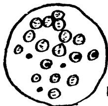
Fig. 3. Schematic drawings of three Condition Factors and their qualitative determination. C = unaffected; T = affected; T or C requires reference to spawning stage or other factors for better qualification.
