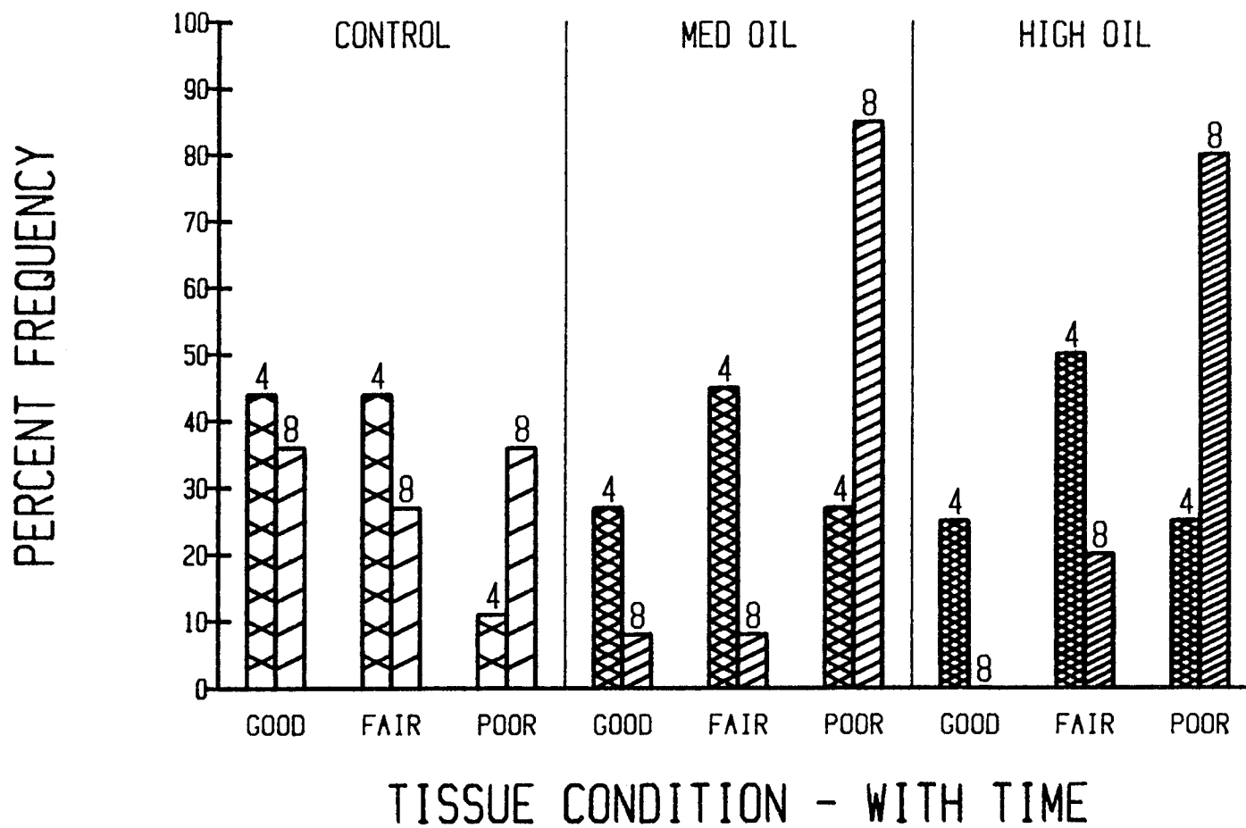
Fig. 12. Comparison of study populations to show percent frequency of animals in Good, Fair, or Poor condition in the 4-5 week period (4) and 8-9 week period (8).
