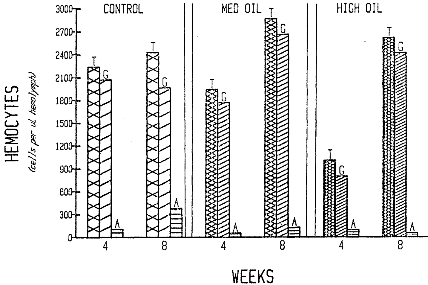
Fig.5. Population mean absolute values from differential cell counts to show changes in types as a result of time and exposure to 500 and 1000 nL/L of oil. Control, Medium oil and High oil mean total cell counts (T) compared to mean granulocytes (G) and agranulocytes (A) examined in 4-5 weeks (4) and 8-9 weeks (8).
