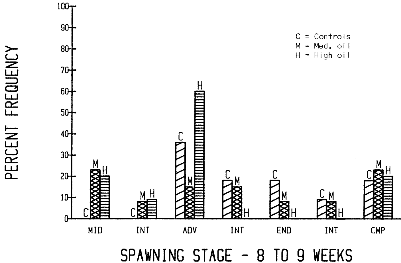
Fig. 10. Comparison of study populations to show frequency of animals in each spawning stage. MID = Mid Spawning; INT. = Inter-stage; ADV. = Advance Spawning; END = End Spawning; CMP = Completed Spawning.
