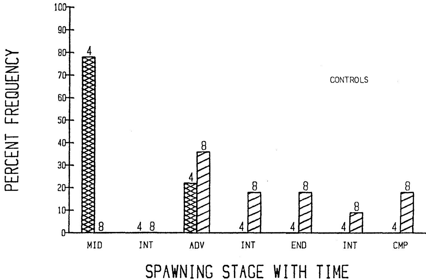
Fig. 8. Percent frequency of controls in spawning stages showing changes occurring with time. MID = Mid Spawning; INT. = Inter-stage; ADV. = Advance Spawning; END = Spawning; CMP = Completed Spawning. 4-5 week period (4) and 8-9 week period (8).
