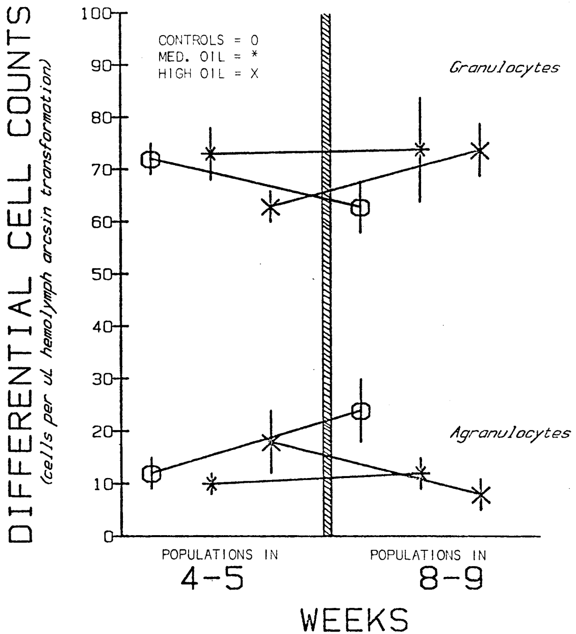
Fig. 4. Percentages of differential hemocytes as a result of time and exposure to 500 and 1000 nL/L of oil. Population means and 95% confidence for granulocytes and agranulocytes in 4-5 weeks and 8-9 weeks. Number of animals sampled: Controls = 9,11; Med. oil = 11,12; High oil = 4,5.
