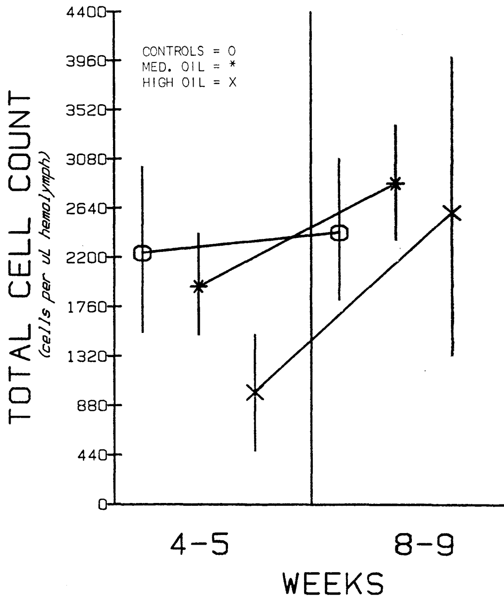
Fig. 6. Mean total cell counts and 90% confidence for each population in two time periods. Changes in total numbers of circulating hemocytes as a result of time and exposure to 500 and 1000 nL/L oil. Number of animals sampled: Controls = 9, 11; Medium Oil = 11, 12; High Oil = 4, 5.
