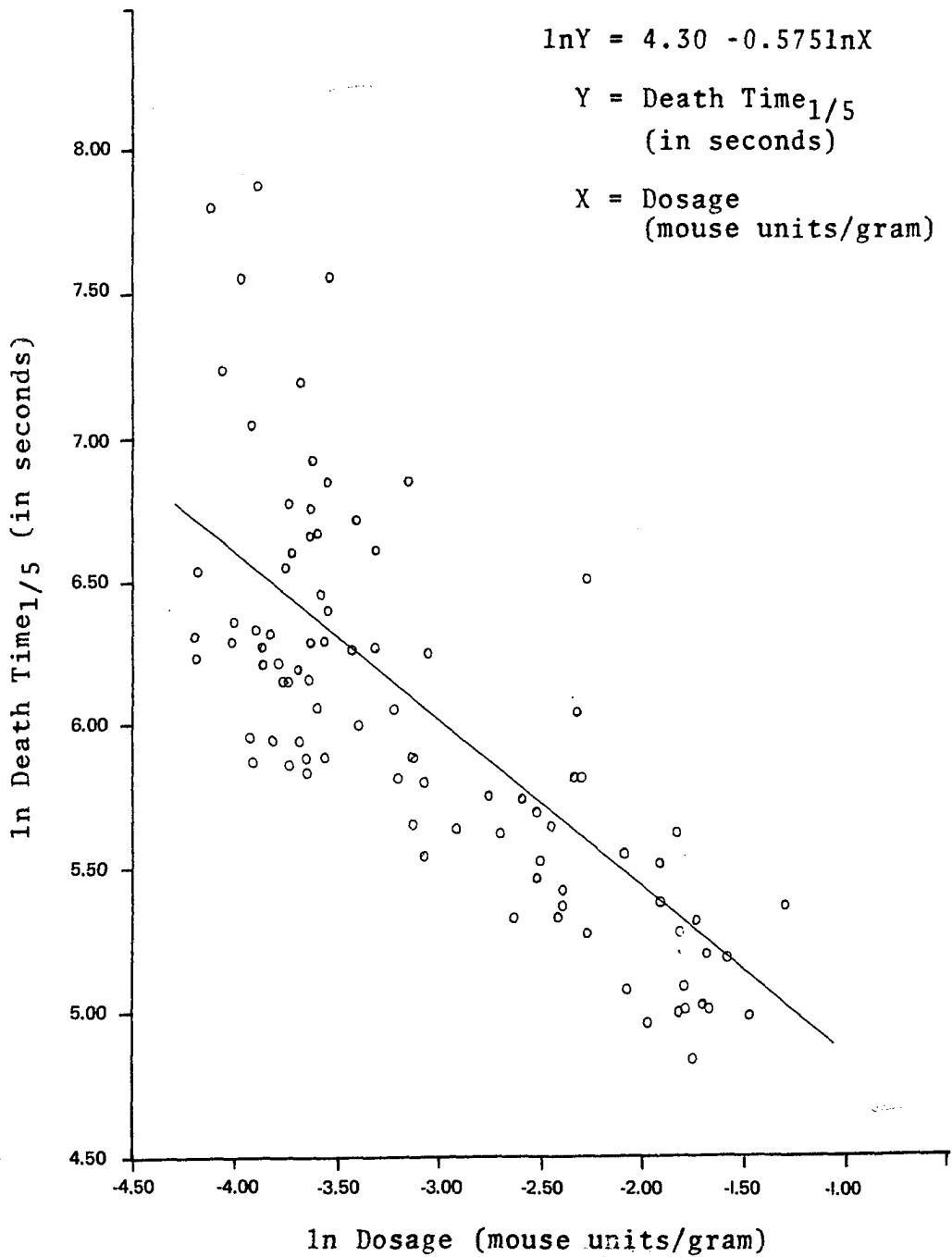
FIGURE 2. Relationship between ln Dosage and ln Death Time 1/5 for Leptocottus armatus . r = .770; p < 0.001 .
