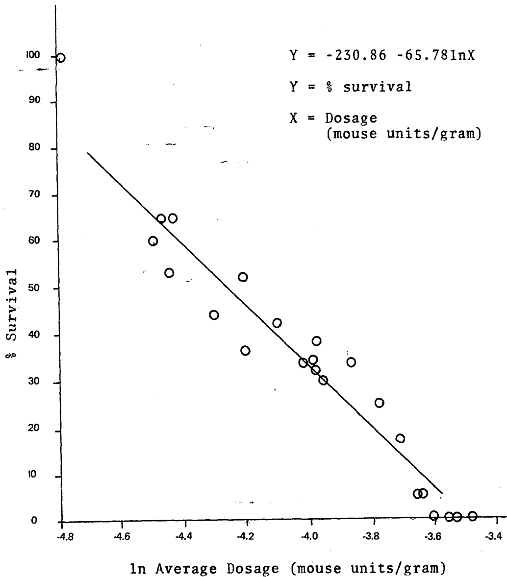
FIGURE 1. Relationship between per cent survival and ln average dosage for groups of Leptocottus armatus . r = .881 ; p < .001
