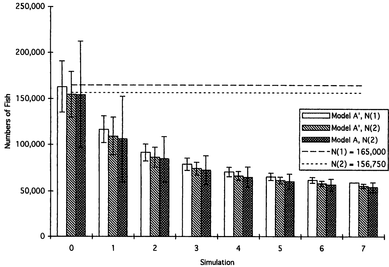
Figure 16. Scenario D estimates (heterogeneity at all sites, with the day group [higher p ] 1/3rd the size of the night group).
