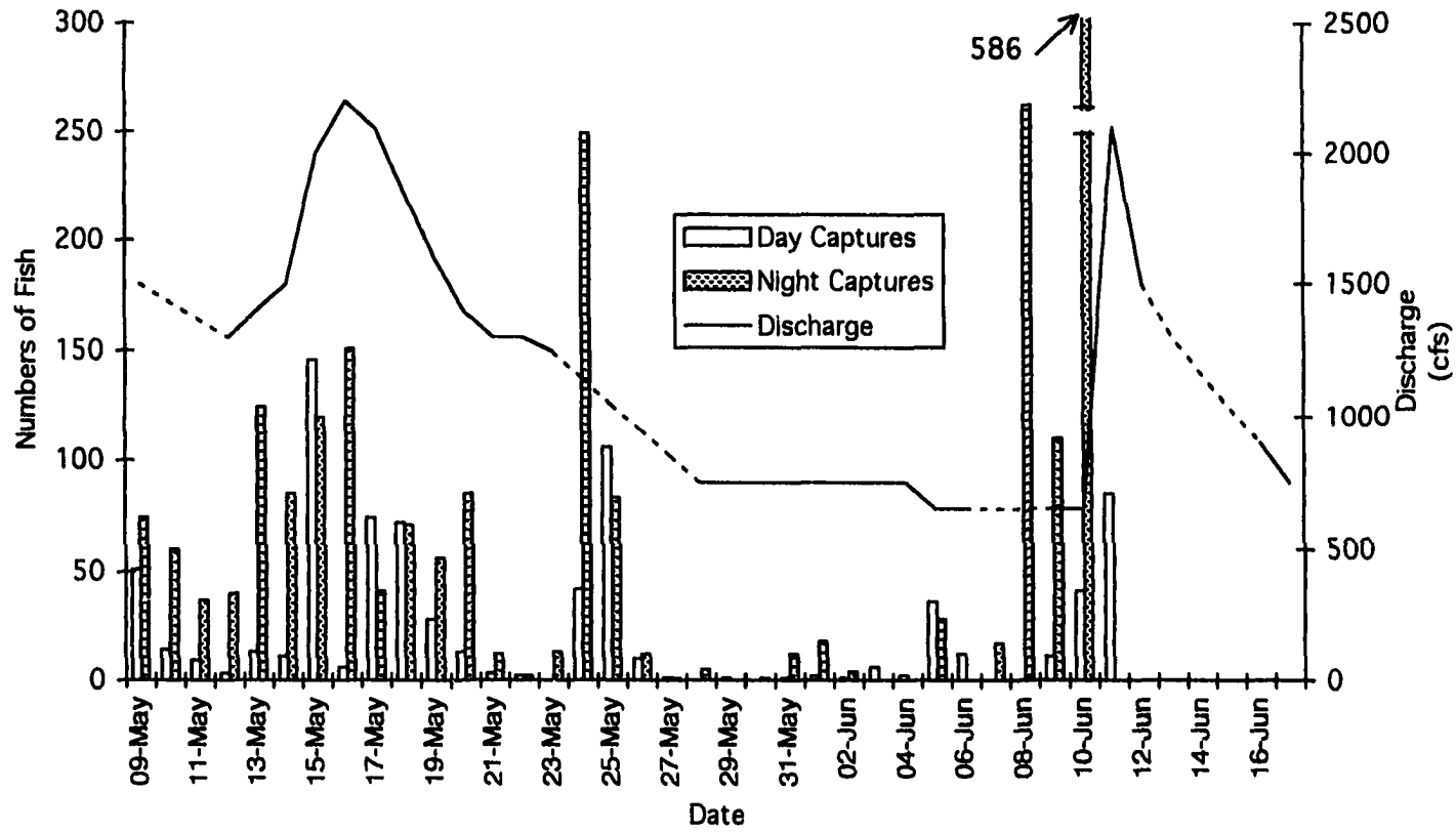
Figure 10. Day and night chinook captures at the middle site, 1997, and discharge. Discharge was measured by the U.S. Army Corps of Engineers at the dam. Dashed lines represent no data taken.
