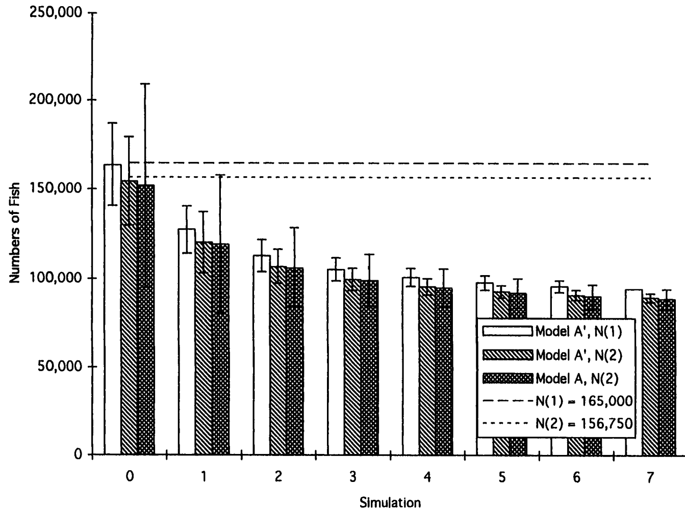
Figure 15. Simulation abundance estimates under Scenario C (heterogeneity at all sites, equal-size subpopulations).
