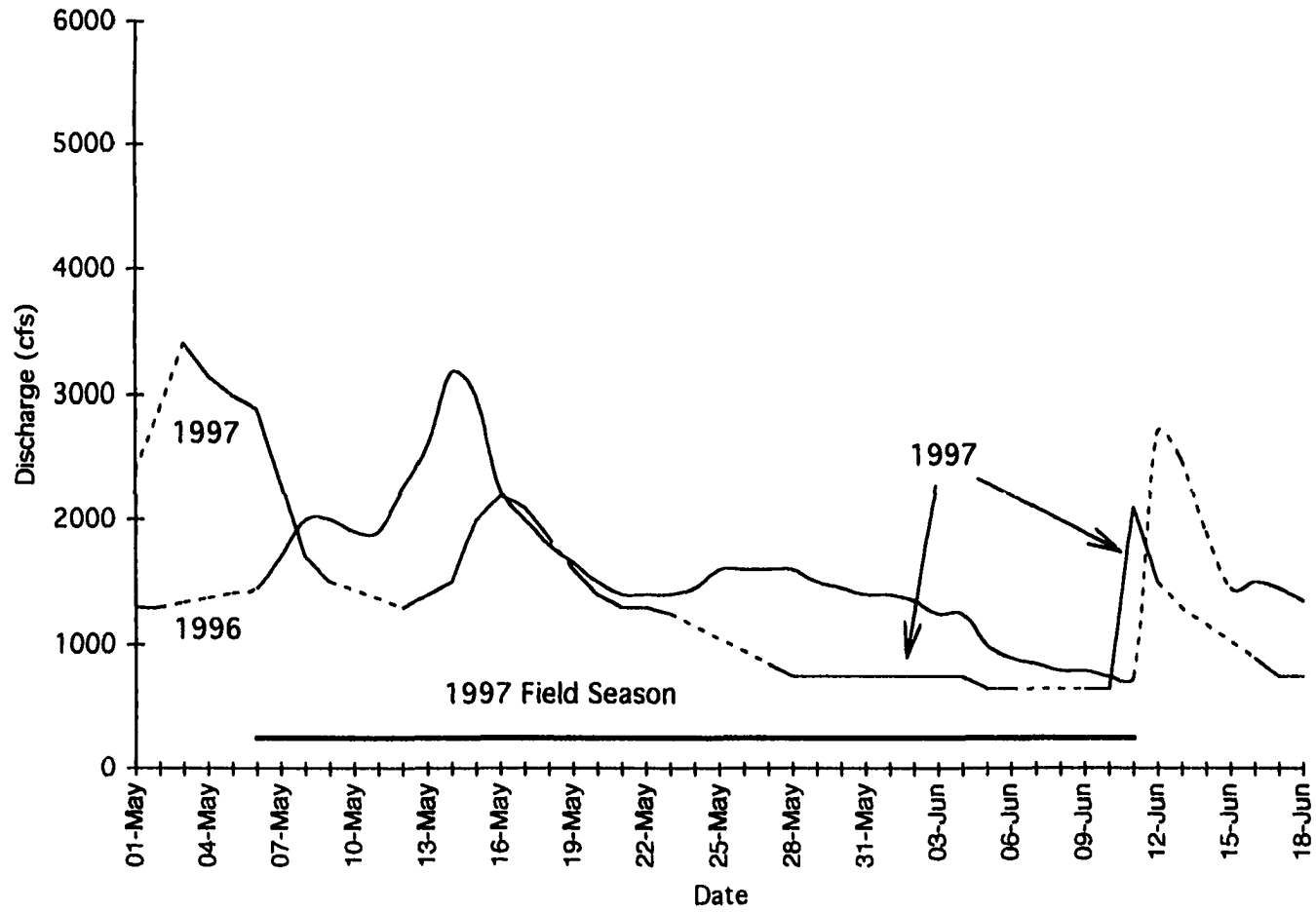
Figure 5. Discharge at the Chena River Dam in May and early June, 1996 and 1997. The dashed lines represent no data recorded.
