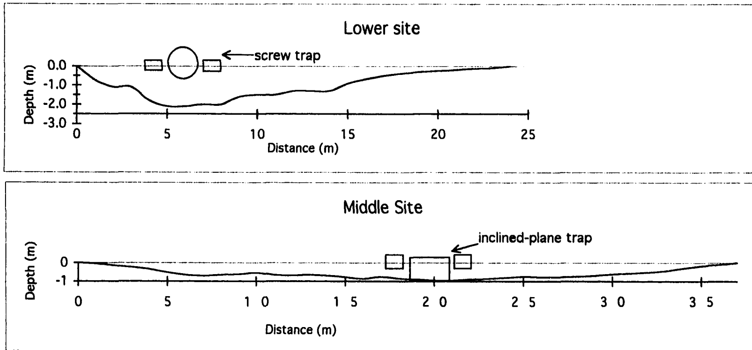
Figure 8. Depth profiles at the lower and middle sites, looking downstream, on June 7th, 1997.
