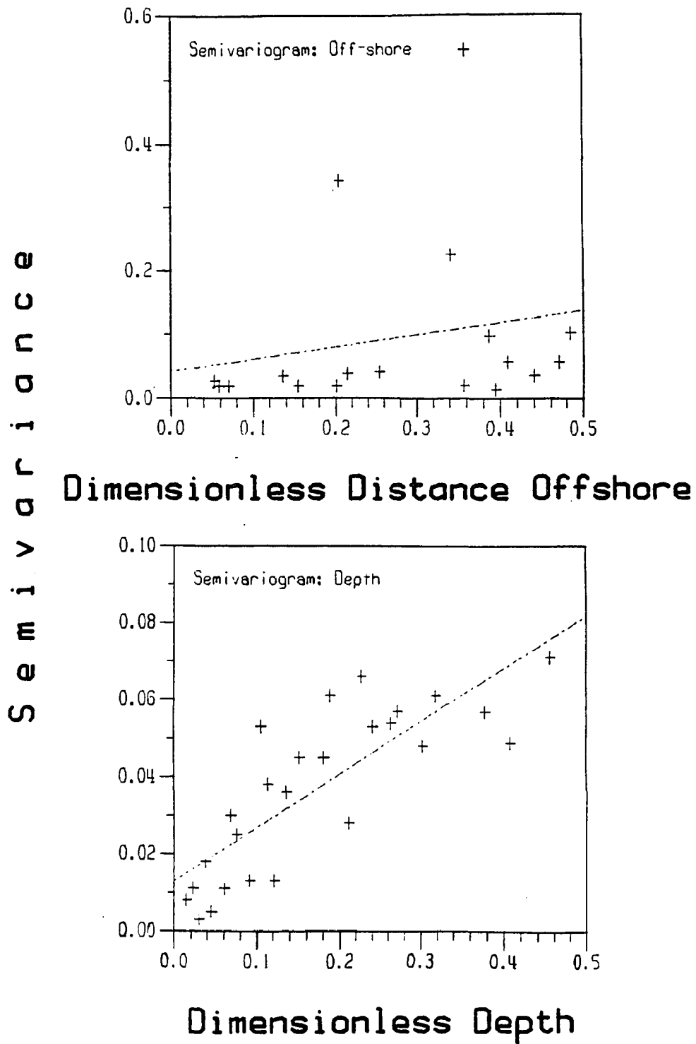
Figure 6-10. Semivariogram of \sigma_t versus distance offshore and depth.
