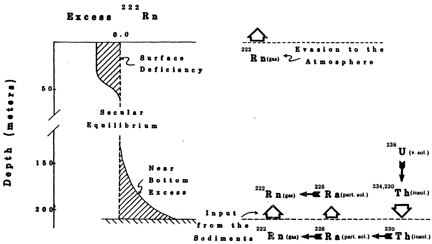
Figure 1-1. Ideal ocean radon profile. Over most of the water column 222 Rn is in radioactive equilibrium with its parent 226 Ra. Near the surface the deficiency in 222 Rn is caused by evasion to the atmosphere. Near the bottom an excess of 222 Rn is caused by input from the sediments. A portion of the 238 U decay series and the important properties of the members is also shown.
