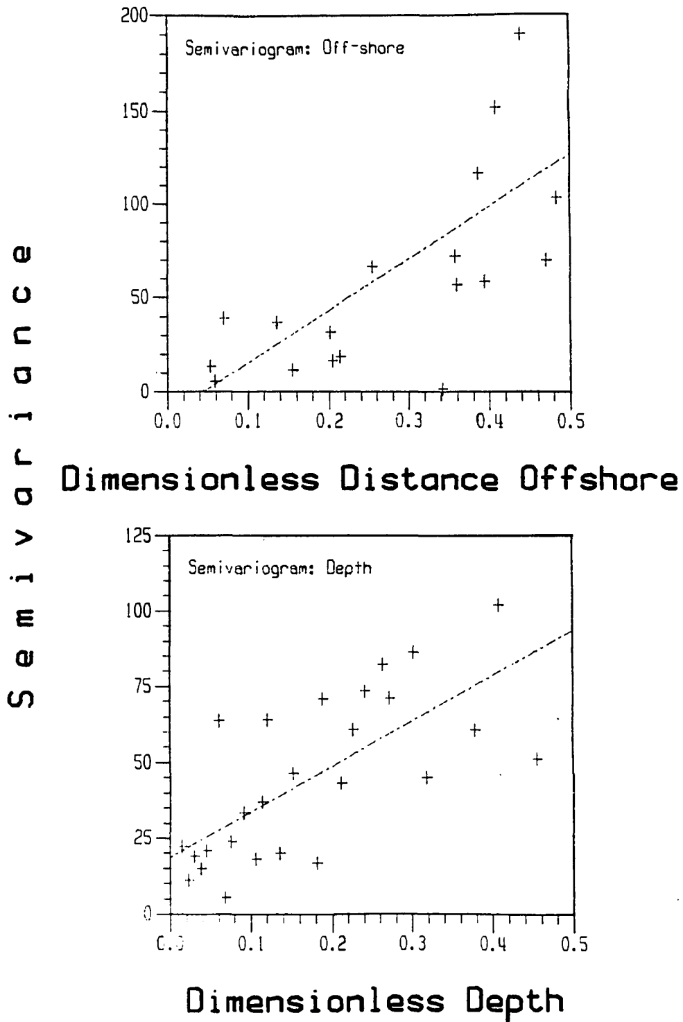
Figure 6-8. Semivariogram of total ^{222}\text{Rn} versus distance offshore and depth.
