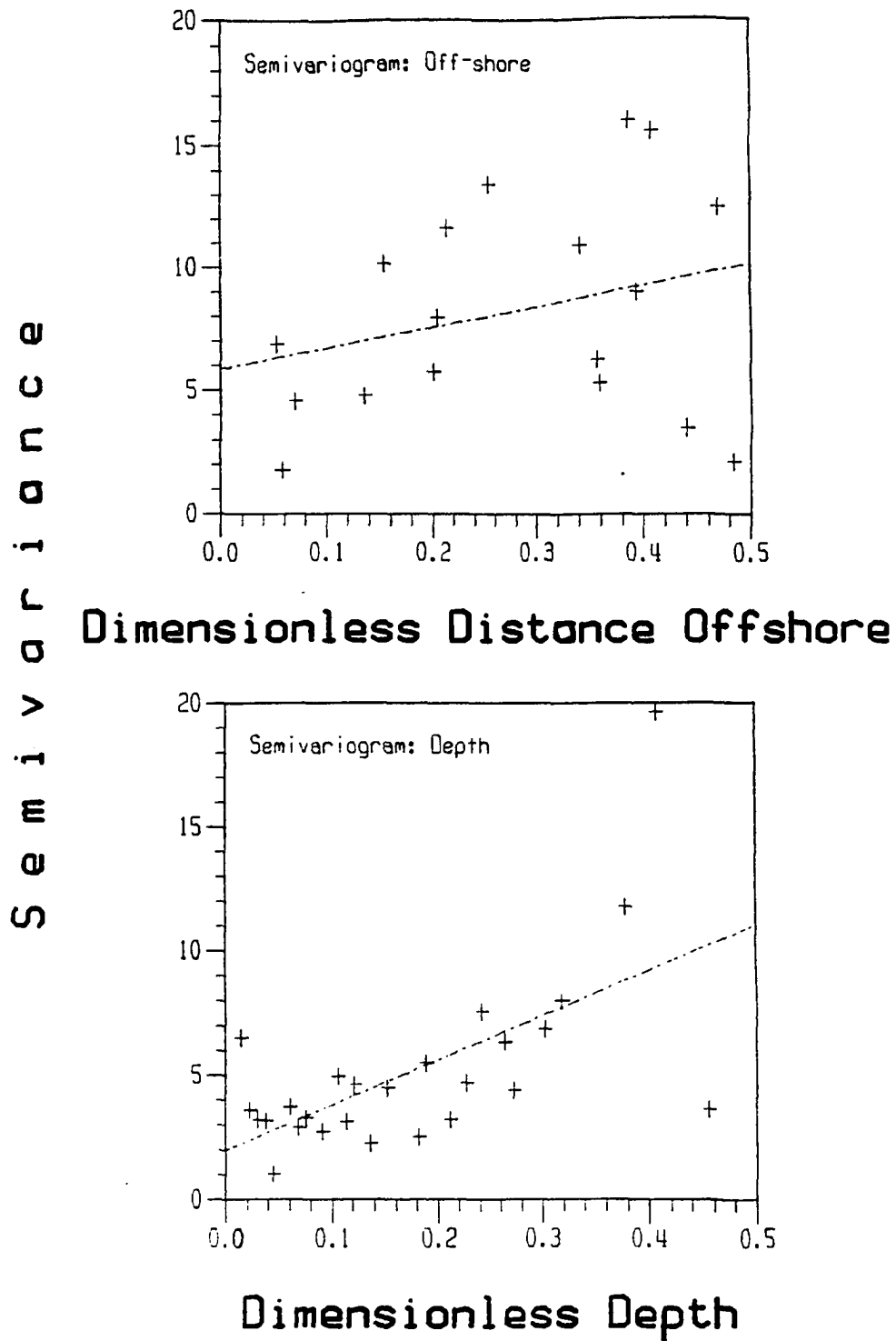
Figure 6-9. Semivariogram of ^{226}\text{Ra} versus distance offshore and depth.
