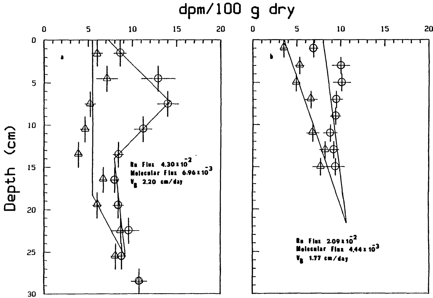
Figure 4-4. Radon-222 and 226 Ra depth distributions in sediment cores. The actual flux exceeds the molecular flux (atoms cm -2 sec -1 ). a) Station HX028-0120, 110 m. b) Station HX048-0014, 129 m. \Delta 222 Rn, \circ 226 Ra.
